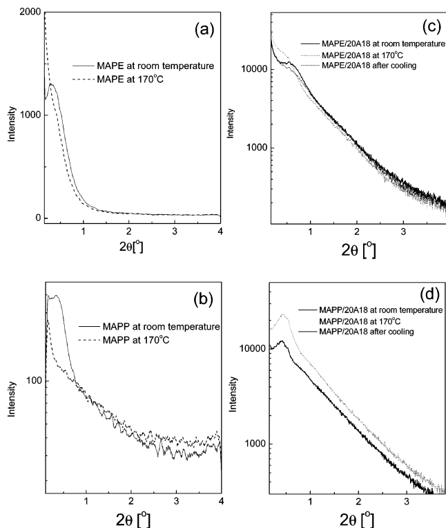
Figure 1. SAXS patterns of (a) MAPE, (b) MAPP, (c) MAPE/20A18 fiber, and (d) MAPP/20A18 fiber at room temperature and above melting temperature of matrix polymer.
