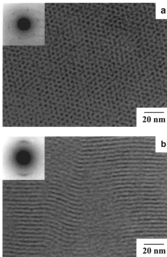
Figure 2. TEM micrographs of (a) homeotropically and (b) planar aligned \Phi_h LC assembly generated by supramolecular cylinders self-assembled from 1 . Insets are electron diffraction patterns obtained from these specimens.
